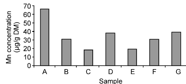
Fig 2: Distribution of Mn in samples: A- Soil; B- Agaricus biosporus ; C- Polyporus frondosis ; D- Armillariella mellea ; E- Pleurotus sapidus ; F- Polyporus sulphureus ; G- Pleurotus ostreatus
