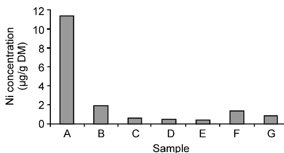
Fig. 4: Distribution of Ni in samples: A- Soil; B- Agaricus biosporus ; C- Polyporus frondosis ; D- Armillariella mellea ; E- Pleurotus sapidus ; F- Polyporus sulphureus ; G- Pleurotus ostreatus
