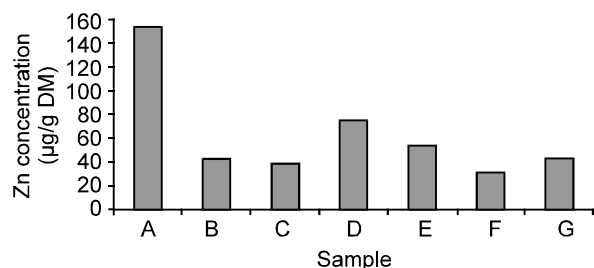
Fig. 1: Distribution of Zn in samples: A- Soil; B- Agaricus biosporus ; C- Polyporus frondosis ; D- Armillariella mellea ; E- Pleurotus sapidus ; F- Polyporus sulphureus ; G- Pleurotus ostreatus
