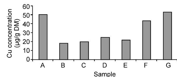
Fig 3: Distribution of Cu in samples: A- Soil; B- Agaricus biosporus ; C - Polyporus frondosis ; D- Armillariella mellea ; E- Pleurotus sapidus ; F- Polyporus sulphureus ; G - Pleurotus ostreatus
