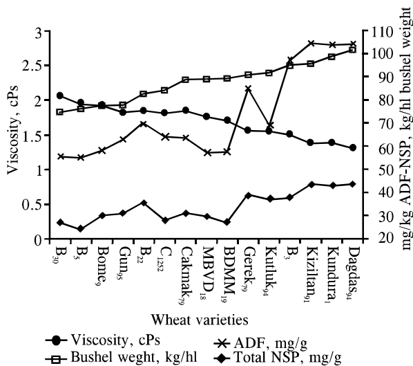
Fig. 1: Correlation (-0.94) between in vitro viscosity and bushel weight of wheat varieties.
