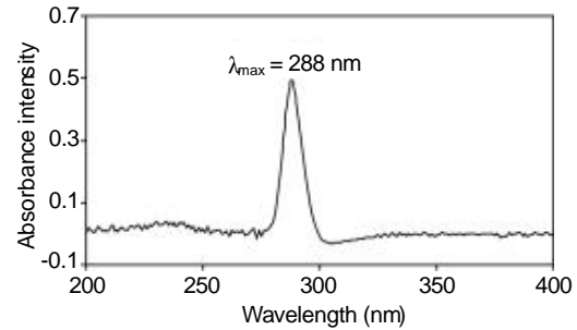
Fig. 1: Absorbance pattern of standard caffeine
