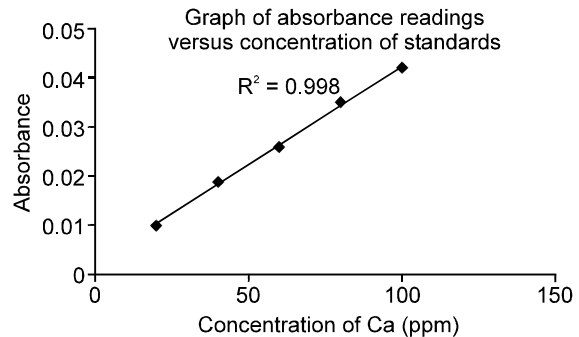
Fig. 3: Calibration graph for Ca standards
