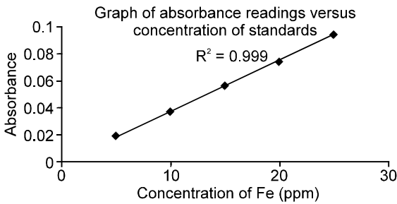
Fig. 5: Calibration graph for Fe standards
