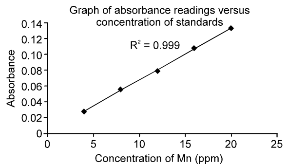
Fig. 4: Calibration graph for Mn standards
